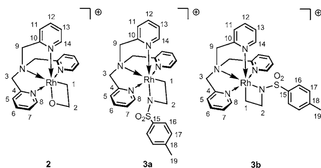
Figure 1. Comparison of ^1\text{H} NMR spectral data of 2 and 3a (600 MHz, \text{CD}_2\text{Cl}_2 , 298 K, with a \text{Cl}^- counterion).
