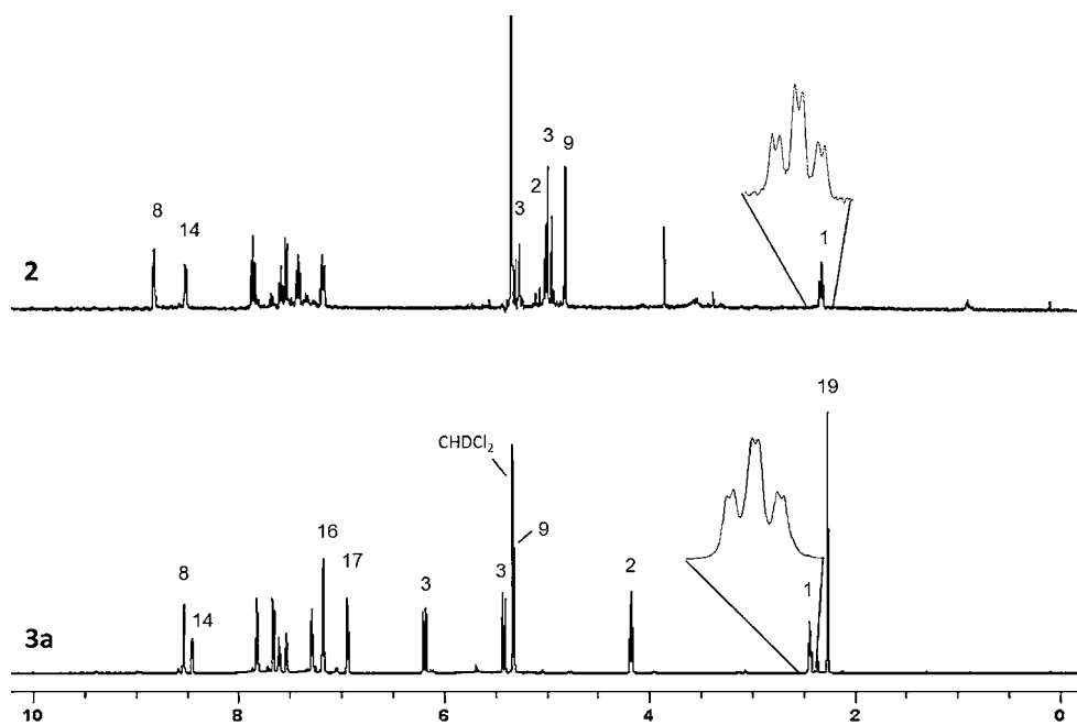
Figure 1. Comparison of ^1\text{H} NMR spectral data of 2 and 3a (600 MHz, \text{CD}_2\text{Cl}_2 , 298 K, with a \text{Cl}^- counterion).
